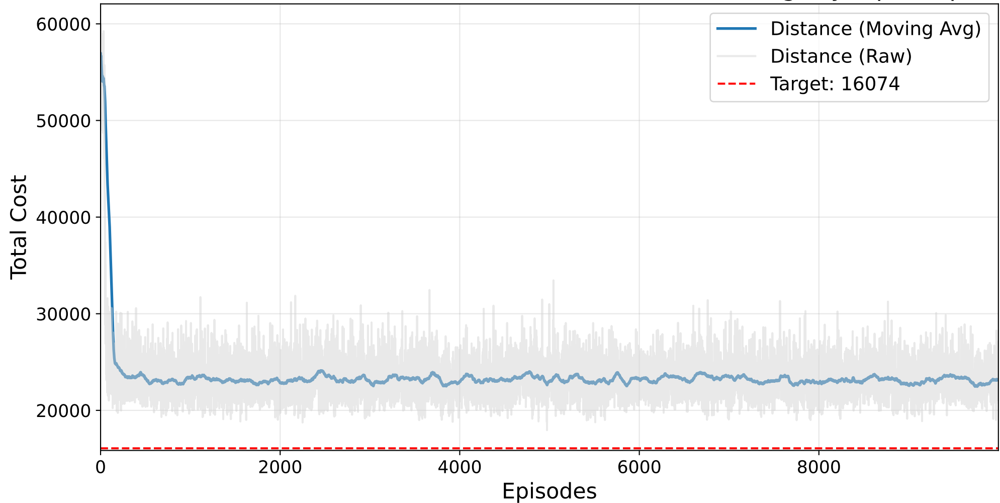
Final GAUSSIAN PROCESS Masked AutoRL-SOP Training - ry48p.2.sop
